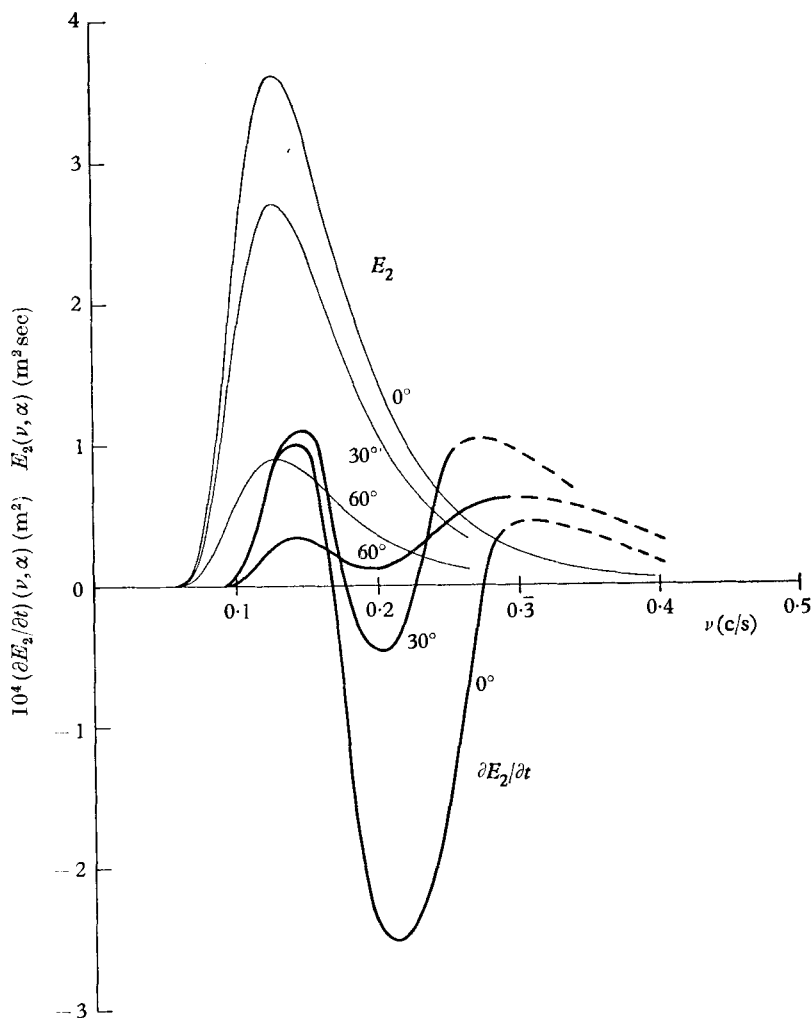
FIGURE 1. Energy transfer for a Neumann spectrum with \cos^2 \alpha -spreading factor. (Wind velocity: 10 \text{ m/s} = 19.4 \text{ knots} .)
