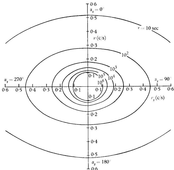
FIGURE 4. Decay time \tau for swell travelling through a Neumann spectrum (wind velocity: 10 m/s, spreading factor: \cos^2 \alpha ). The mean direction of the spectrum is upwards ( \alpha_s = 0 ); the spectral peak is at 0.125 c/s.
